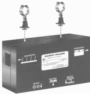
FIGURE 14 Clipping Humidistat to Dehumidifier
