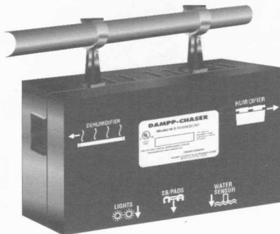
FIGURE 14 Clipping Humidistat to Dehumidifier
