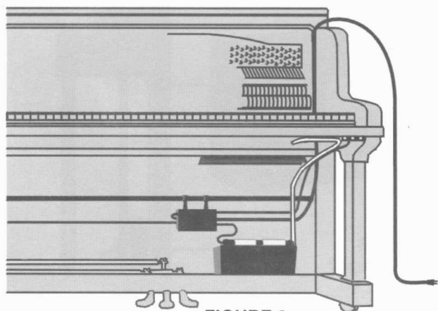
FIGURE 3 Humidifier placement
